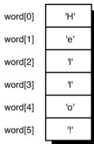
Figure 9.1 The array word in memory.
