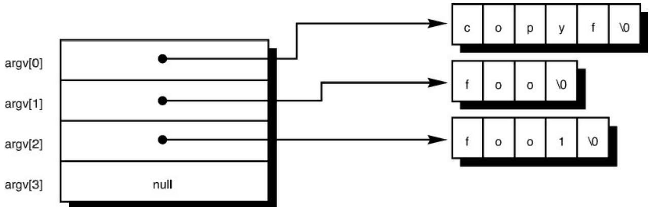
Figure 16.1 argv array on startup of copyf .
