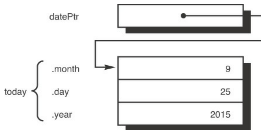
Figure 10.2 Pointer to a structure.
