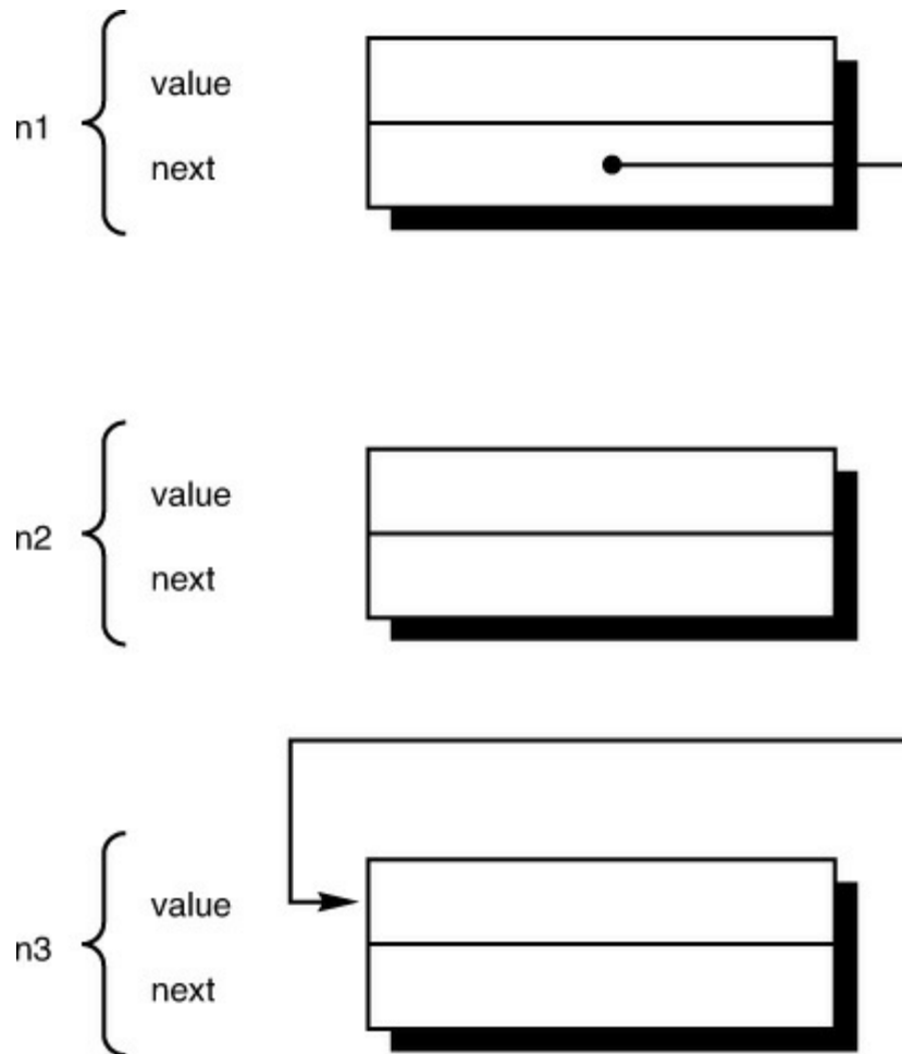
Figure 10.6 Removing an entry from a linked list.
