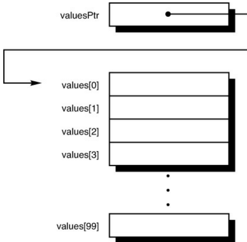
Figure 10.9 Pointer to an array element.
