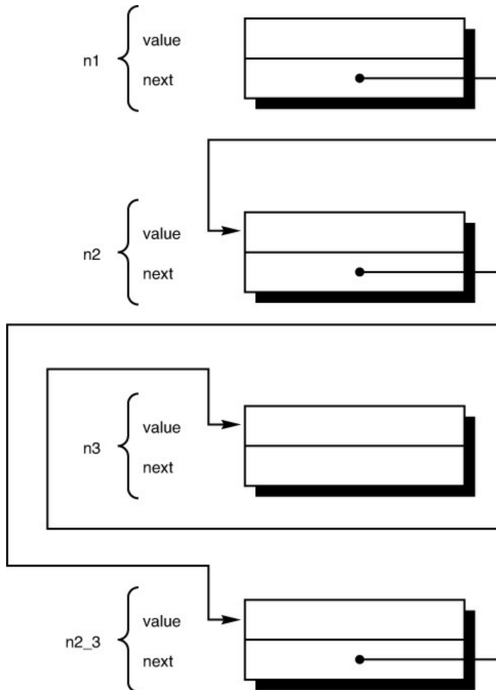
Figure 10.7 Inserting an element into a linked list.
