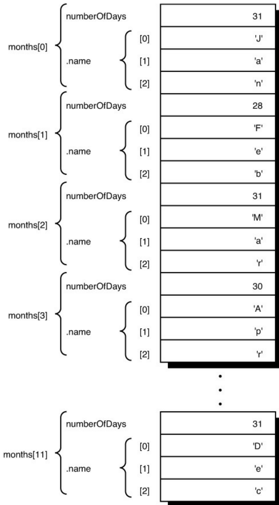
Figure 8.3 The array months .
