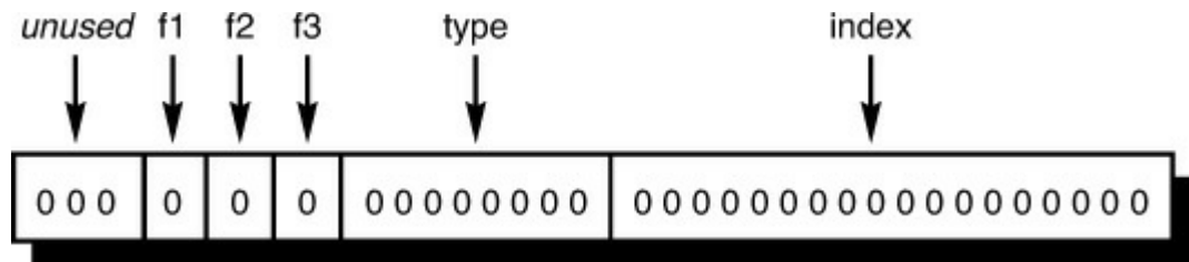
Figure 11.1 Bit field assignments in packed_data .
